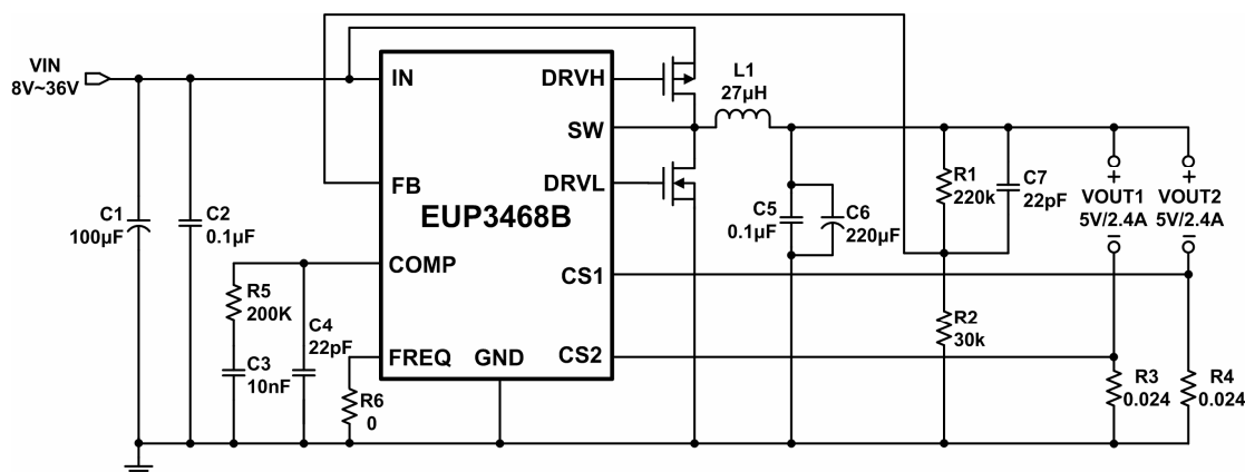
Figure 1. Application Circuit
