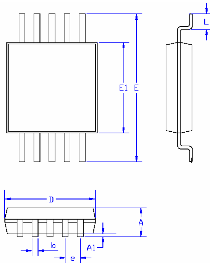
MSOP-10
