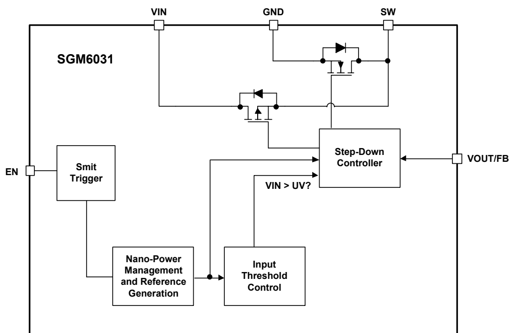
Figure 3. Block Diagram
