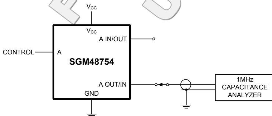
Test Circuit 3. Capacitance
