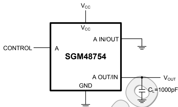
Test Circuit 1. Charge Injection (Q)
