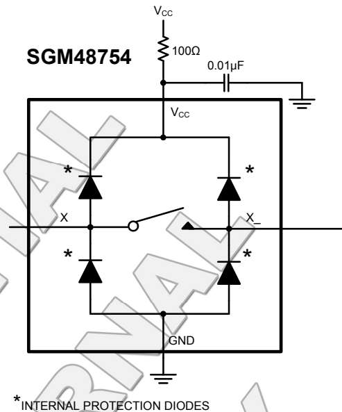
Figure 1. Over-Voltage Protection Using External Resistor
