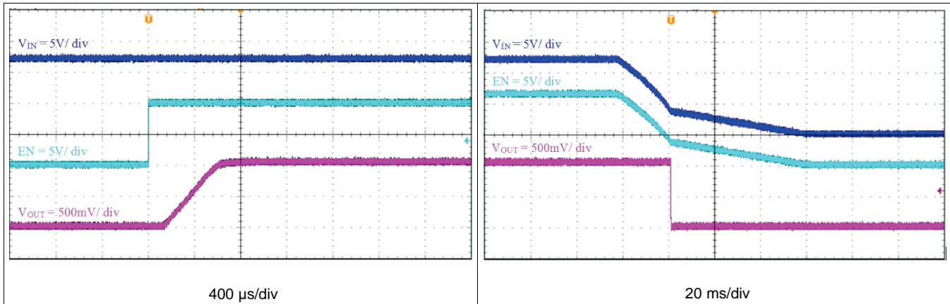
Figure 27. TPS565201 Startup Relative to EN
