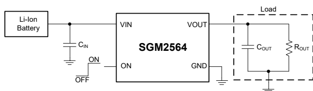
Figure 7. Typical Application Circuit
