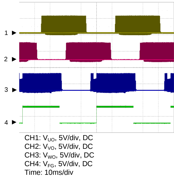
Rotation Mode Waveform (PWM=9)
