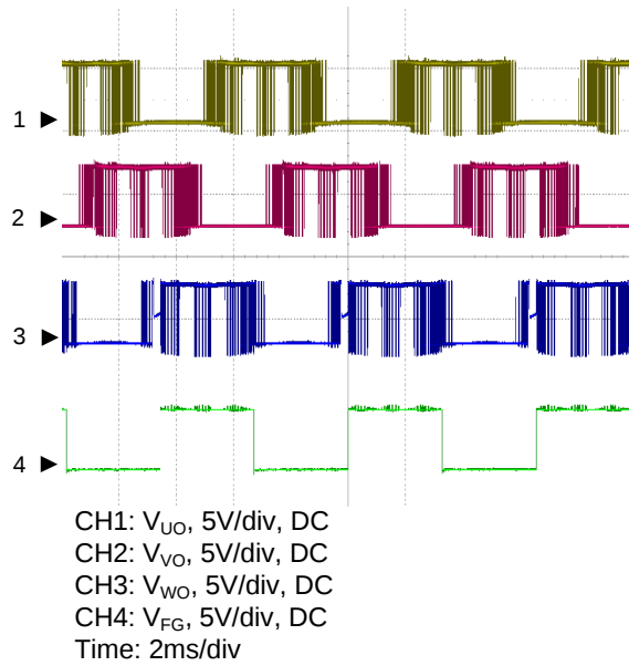
Rotation Mode Waveform (PWM=100)
