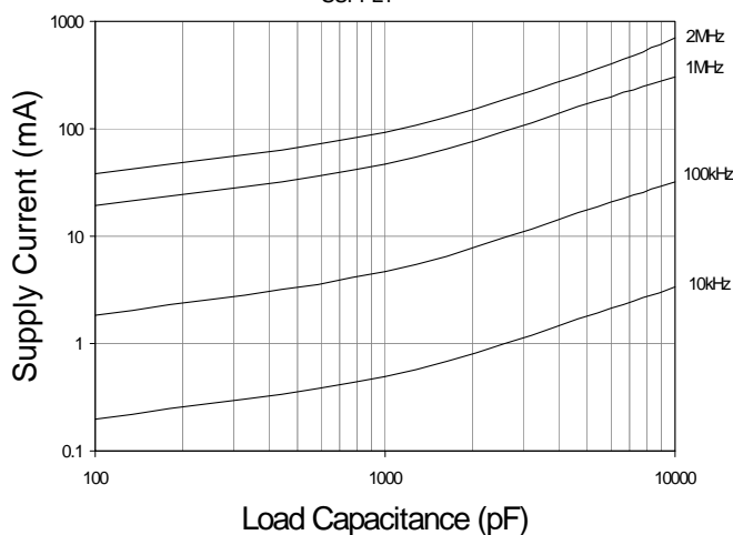
Supply Current vs. Capacitive Load V_{\text{SUPPLY}} = 30V
