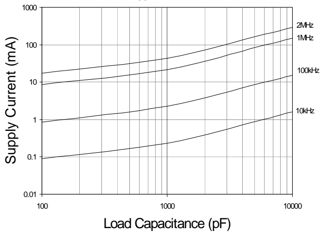
Supply Current vs. Capacitive Load V_{\text{SUPPLY}} = 15V
