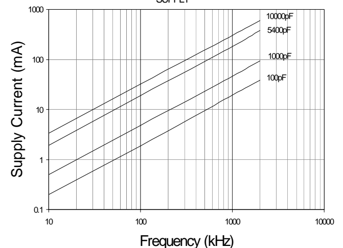
Supply Current vs. Frequency V_{\text{SUPPLY}} = 30V
