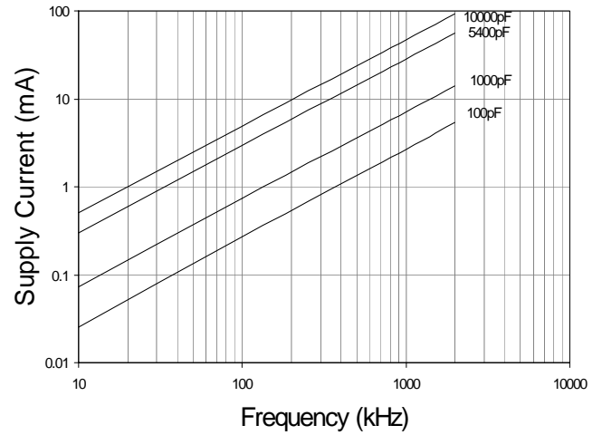
Supply Current vs. Frequency V_{\text{SUPPLY}} = 5V
