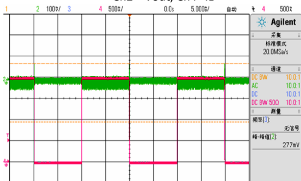
Load Transient
