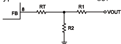
Figure 6: T-Type Network
