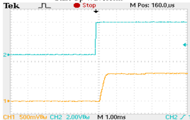
Start Up Waveform
