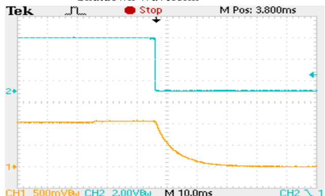
Shutdown Waveform
