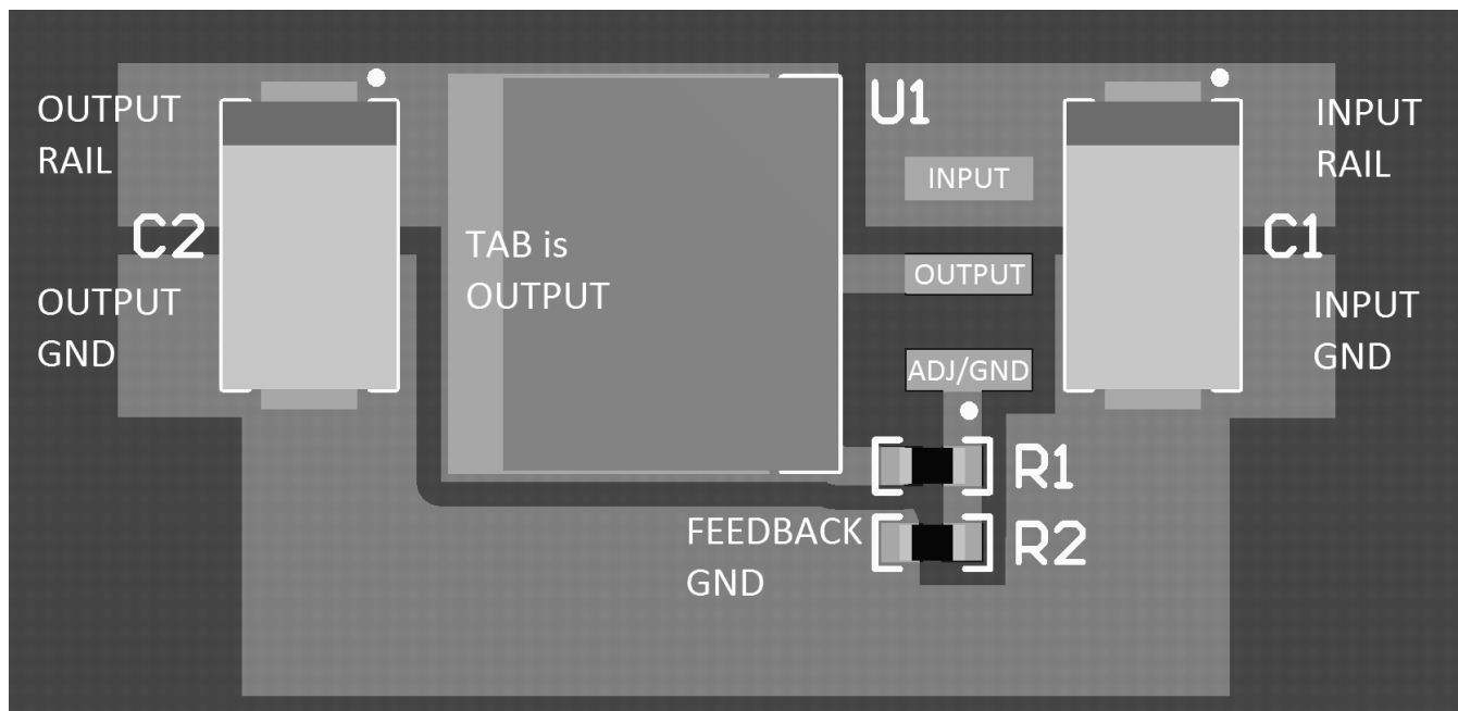
Figure 28. Layout Example
