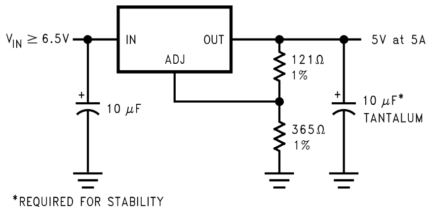
Figure 17. Adjustable @ 5 V
