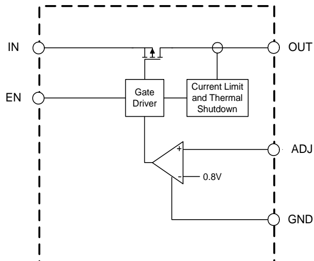
Adjustable Version
