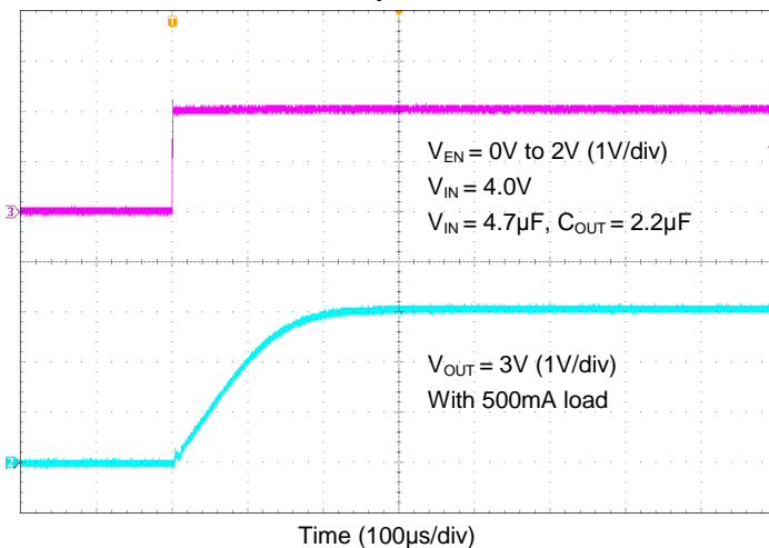
Start-up Time
