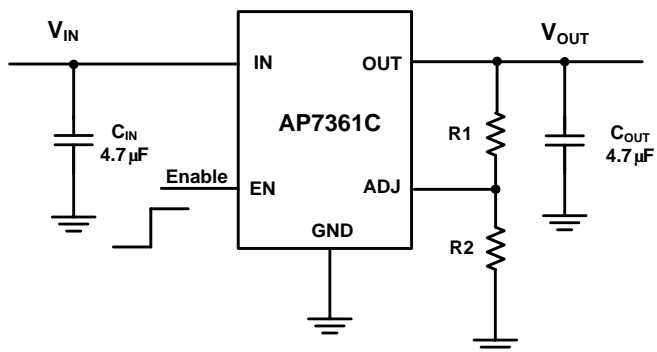
Adjustable Output
