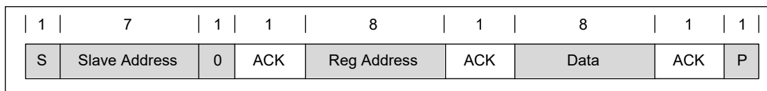
Figure 16. A Single Write Transaction
