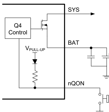
Figure 11. nQON Push Button Circuit
