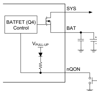
Figure 12. nQON Manual Operation Circuit
