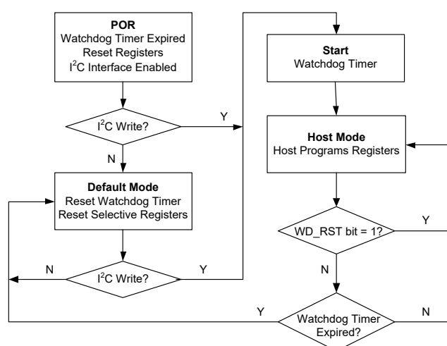
Figure 4. Watchdog Timer Flow Chart
