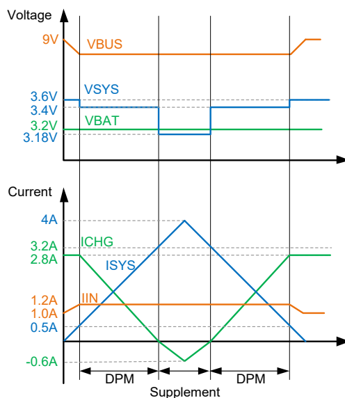
Figure 9. Input, Battery and System Voltage and Currents in DPM
