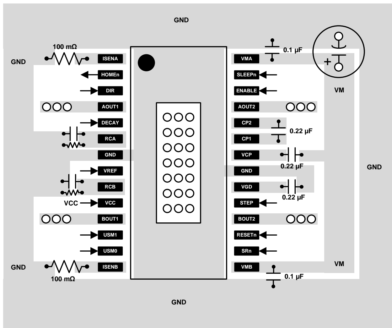
Figure 14. Layout Example Schematic
