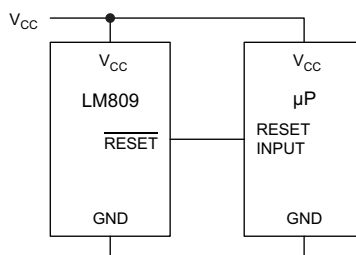
Figure 10. Microprocessor \overline{\text{RESET}} Circuit
