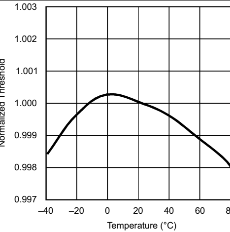
Figure 6. Normalized Reset Threshold vs Temperature
