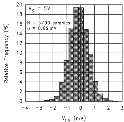
Figure 1. V_{OS} Distribution
