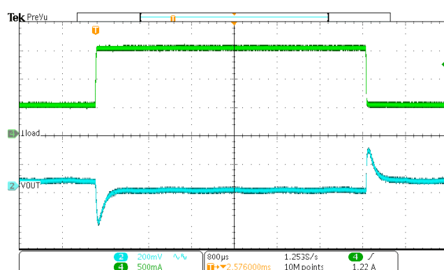
Figure 18. Load Transient VOUT=5V, IOUT=0.5A to 1.5A, SR=250mA/us
