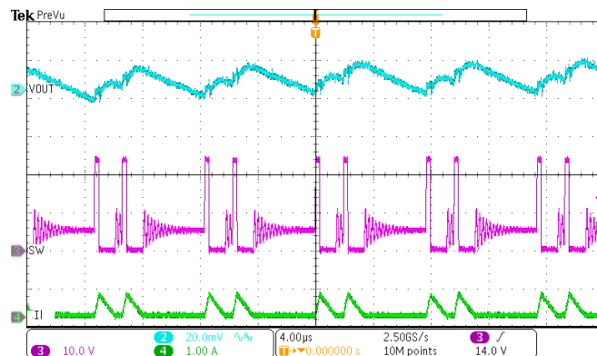
Figure 14. SW node Waveform and Output Ripple VIN=24V, IOUT=100mA
