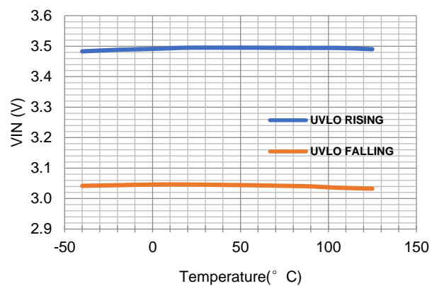
Figure 8. VIN UVLO vs Temperature
