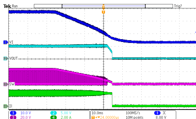
Figure 16. Power Down VIN=24V, VOUT=5V, IOUT=2A
