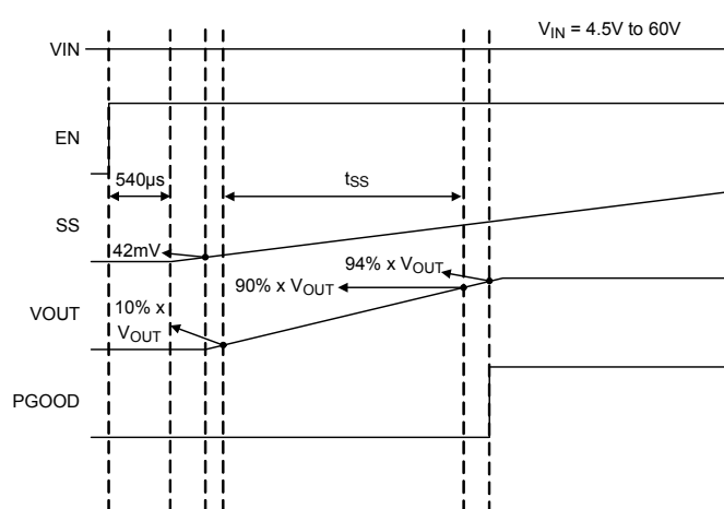
Figure 1 Start-Up Sequence for RT6363GQW
