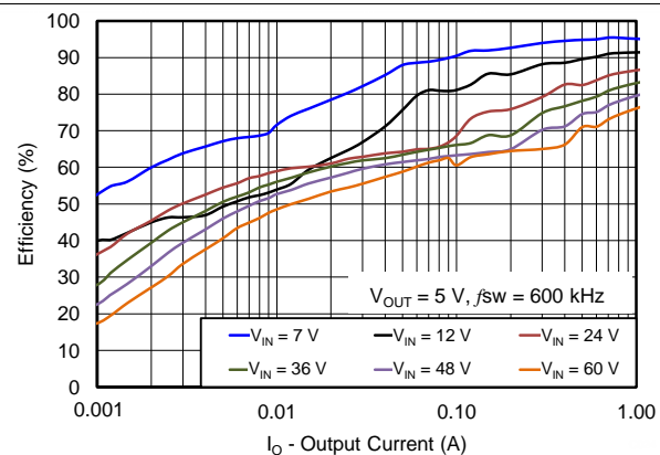
Figure 60. Light-Load Efficiency
