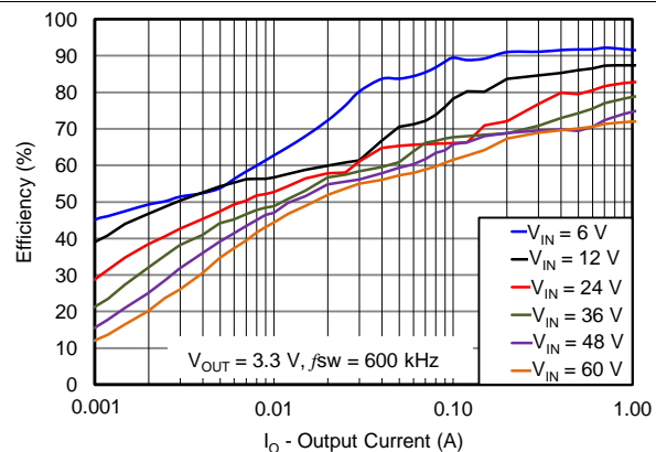
Figure 62. Light-Load Efficiency
