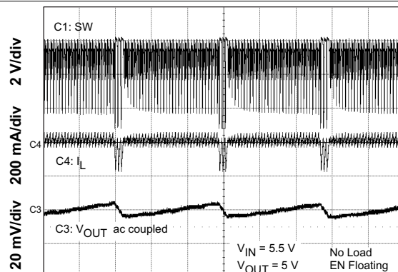
Time = 20 \mu s/div Figure 56. Low-Dropout Operation
