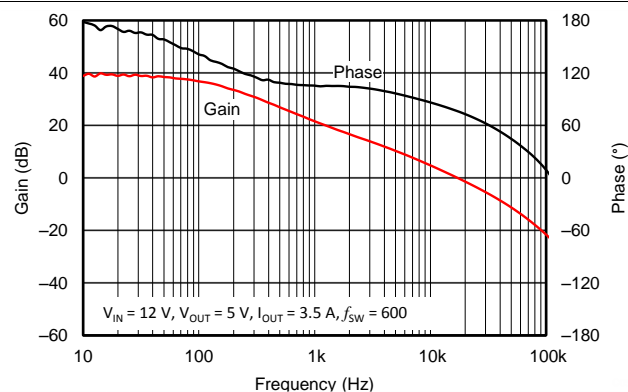
Figure 63. Overall Loop-Frequency Response
