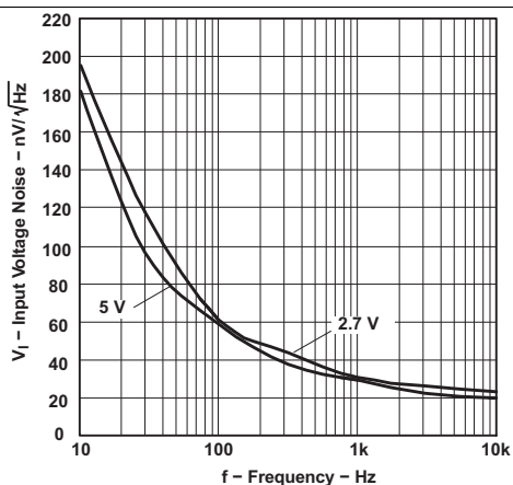
Figure 18. Input Voltage Noise vs Frequency
