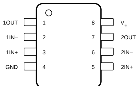
D or DGK Package 8-Pin SOIC or VSSOP Top View
