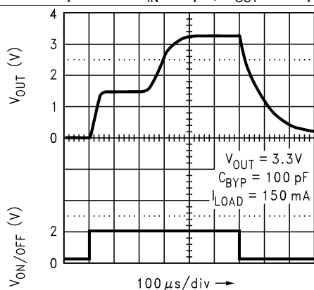
Figure 31. Turnon Time
