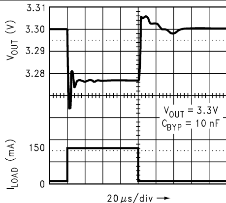
Figure 36. Load Transient Response
