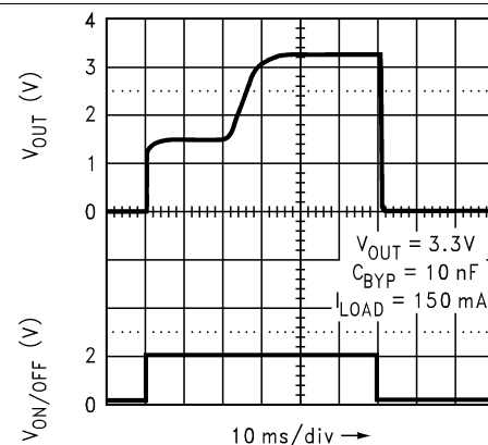
Figure 41. Turnon Time
