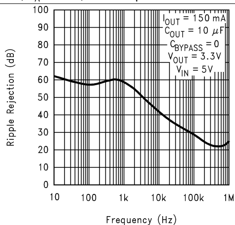
Figure 8. Ripple Rejection
