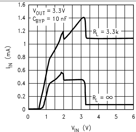
Figure 20. Input Current vs Pin
