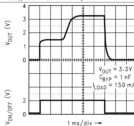
Figure 32. Turnon Time
