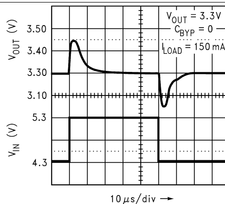
Figure 39. Line Transient Response
