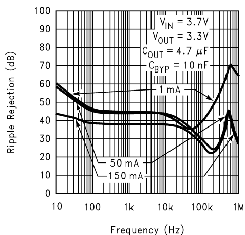
Figure 12. Ripple Rejection
