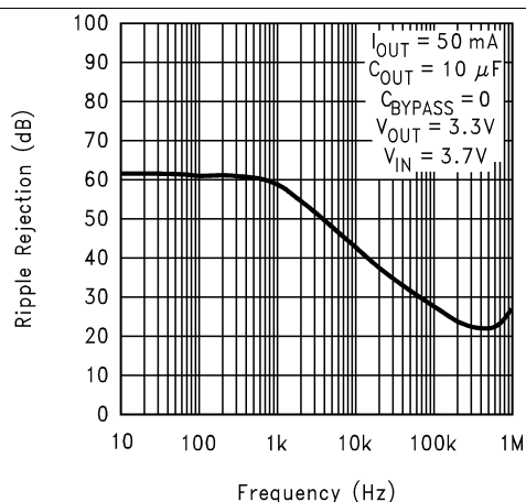
Figure 10. Ripple Rejection
