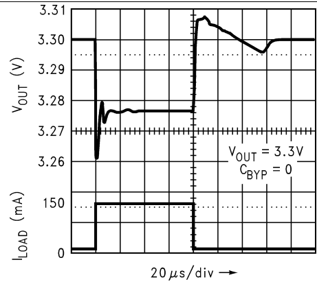
Figure 24. Load Transient Response
