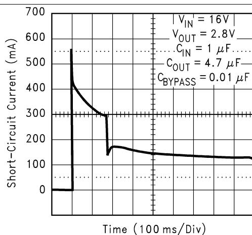
Figure 3. Short-Circuit Current
