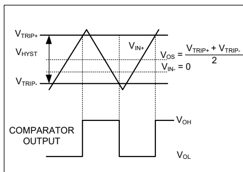
Figure 1. Input and Output Waveform, Non-Inverting Input Varied
