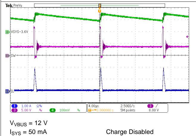
图 34. PFM Switching in Buck Mode
