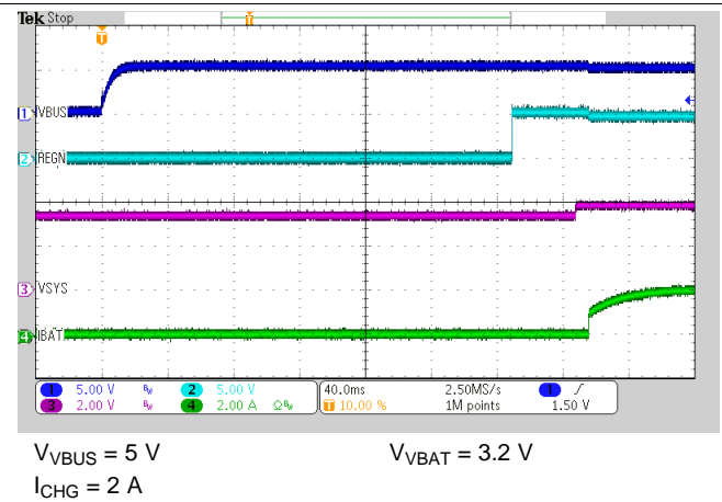
图 31. Power-Up with Charge Enabled
