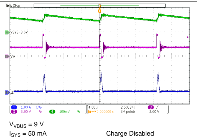
图 33. PFM Switching in Buck Mode
