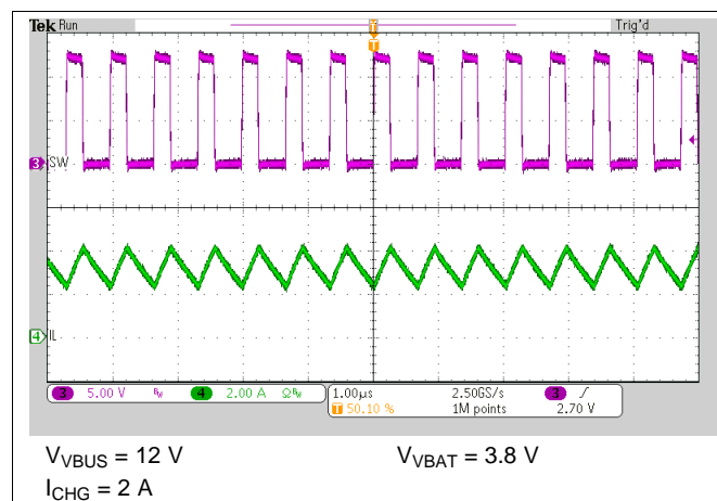
图 36. PWM Switching in Buck mode
