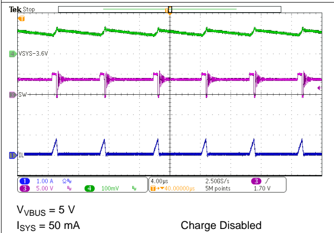
图 32. PFM Switching in Buck Mode
