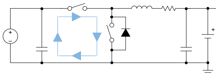
图 50. High Frequency Current Path
