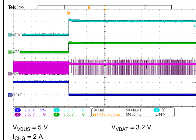
图 38. Charge Disable
