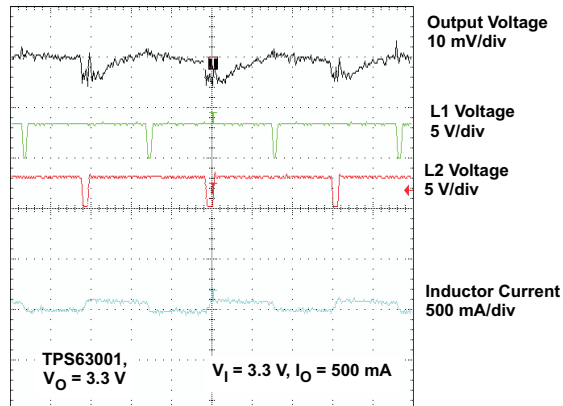
Figure 11. Output Voltage in Continuous Current Mode (TPS63001, V_{IN} = V_{OUT} )
