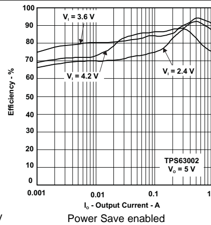
Figure 4. Efficiency vs Output Current (TPS63002)
