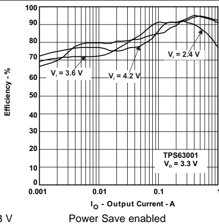
Figure 3. Efficiency vs Output Current (TPS63001)
