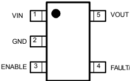
5-Pin SOT-23 (M5) MIC2005-X.XL
