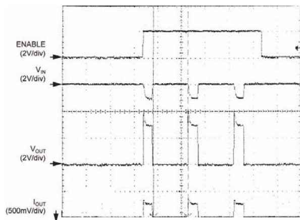
Figure 9. VUVLO Operation
