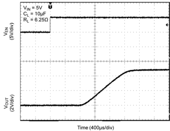
Enable Turn-On/Turn-Off
