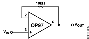
Figure 33. Unity-Gain Follower
