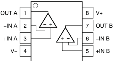
OPA2376: D and DGK Packages 8-Pin SOIC and 8-Pin VSSOP Top View
