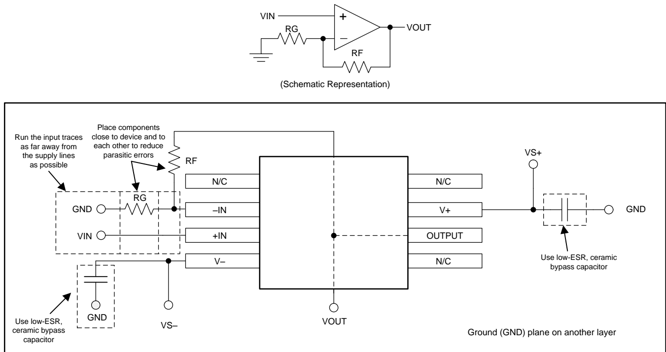
Figure 32. Layout Example
