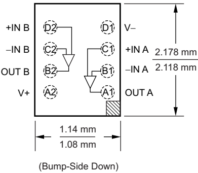
OPA2376: YZD Package 8-Pin DSBGA Top View
