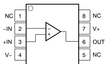
OPA376: D Package 8-Pin SOIC Top View
