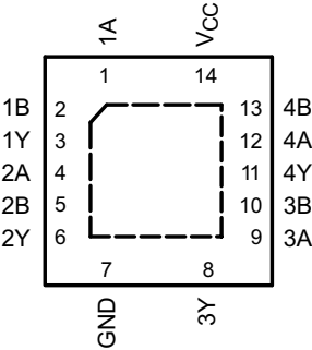
RGY Package 14-Pin VQFN Top View
