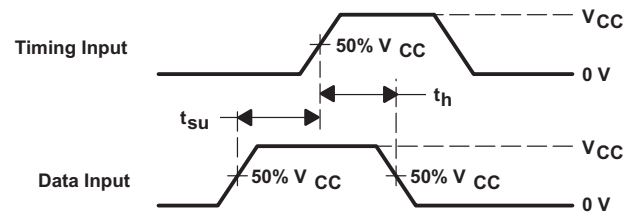
Figure 5. Voltage Waveforms Setup and Hold Times
