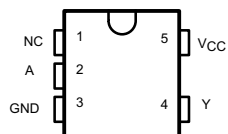
DBV OR DCK PACKAGE (TOP VIEW)
