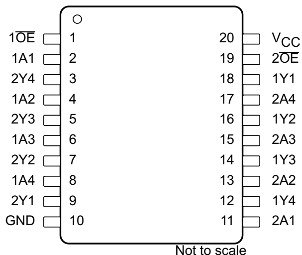
Figure 5-2. DB, DGV, DW, N, NS, and PW Packages 20-Pin SSOP, TVSOP, SOIC, PDIP, SO, and TSSOP Front View
