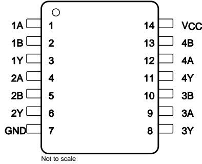
SN54LVC32A J or W Package SN74LVC32A D, DB, NS, or PW Package 14-Pin CDIP, CFP, SOIC, SSOP, SO, TSSOP Top View
