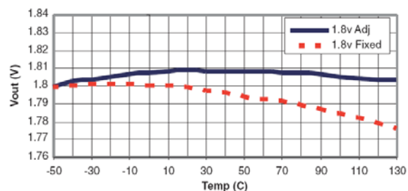
Fig. 10: V_{IN}=3.3V , I_{OUT}=10mA
