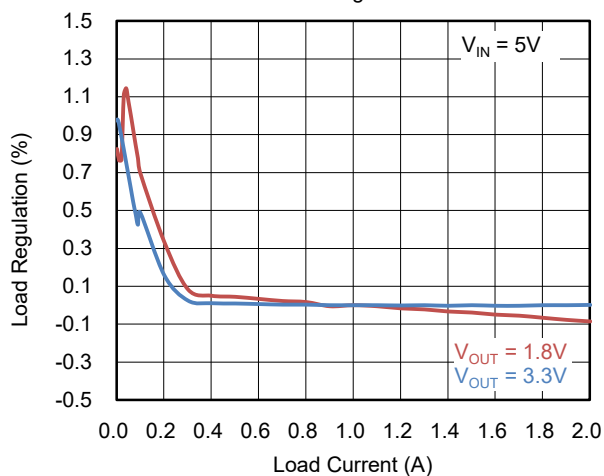
Load Regulation
