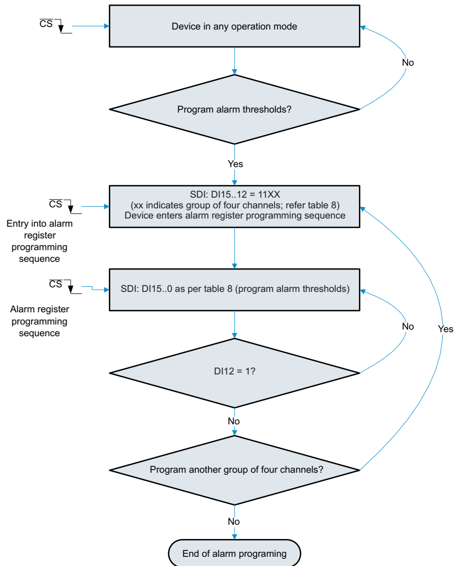
Figure 53. Alarm Program Register Programming Flowchart
