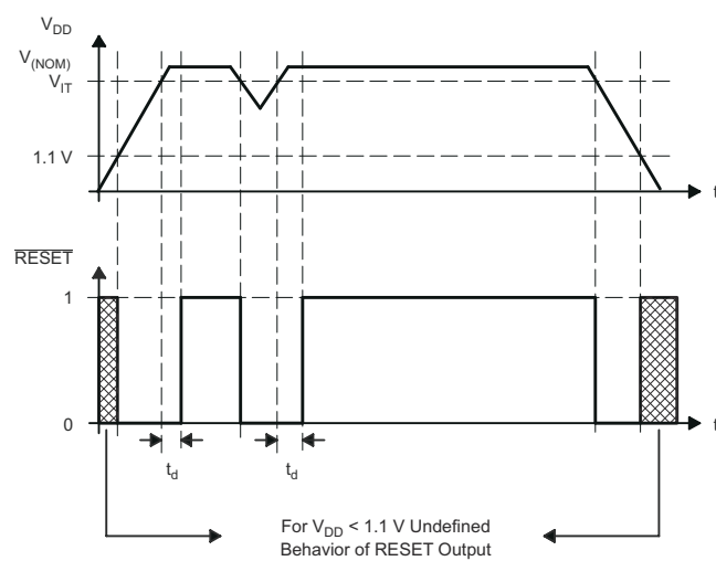
Figure 7-1. Timing Diagram
