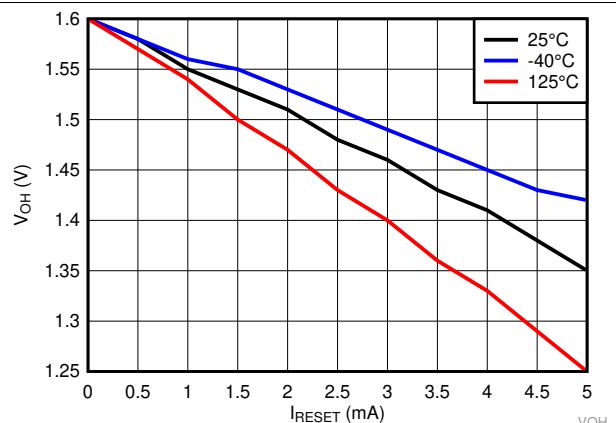
Figure 27. High Level Output Voltage vs I_{\text{RESET}} for TPS3840PH49
