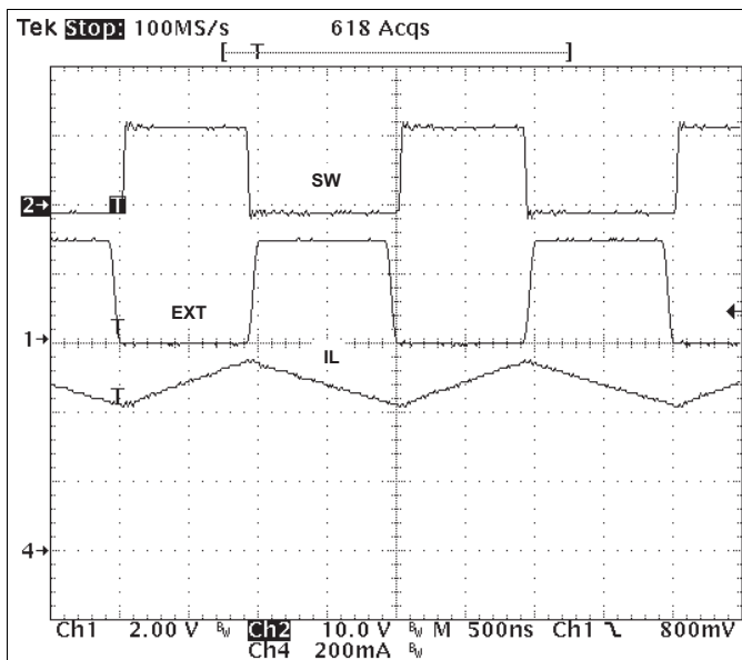
Figure 25. Plot of Synchronizing in CCM
