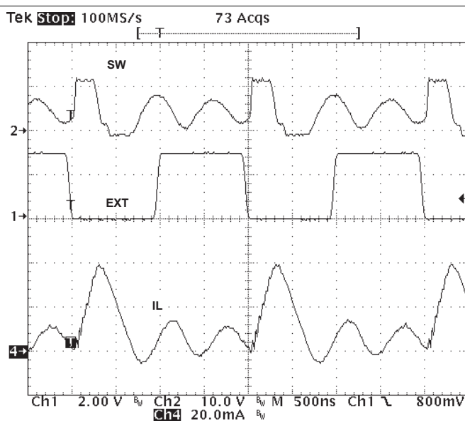
Figure 26. Plot of Synchronizing in DCM
