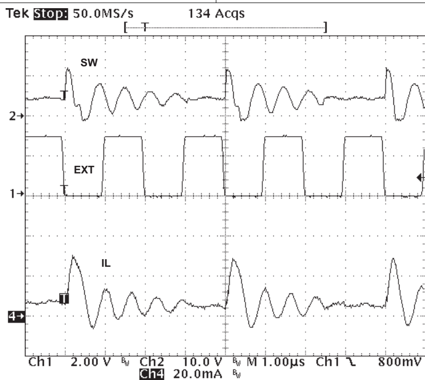
Figure 27. Plot of Synchronizing in Eco-Mode
