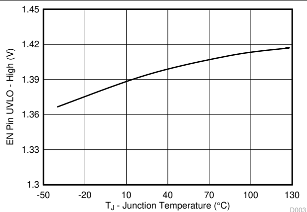
Figure 6-4. EN Pin UVLO High Voltage vs Junction Temperature
