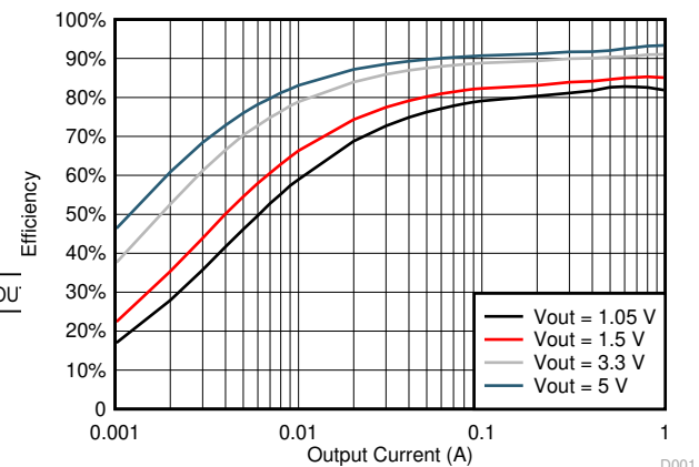
TPS561201 Efficiency
