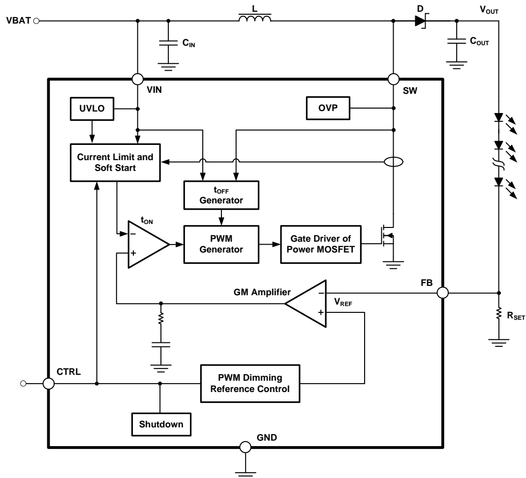
Figure 2. SGM3751 Block Diagram
