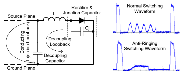
Figure 8. Ringing Cancellation Illustration
