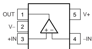
OPA354 DBV Package 5-Pin SOT-23 Top View
