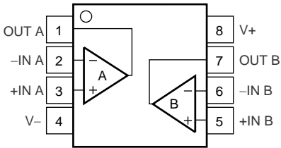
OPA2354 DGK and DDA Packages 8-Pin VSSOP, HSOP Top View
