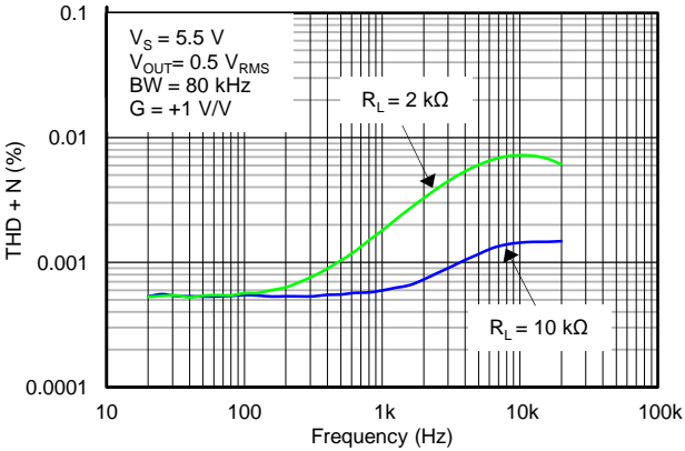
Figure 32. THD+N vs FREQUENCY
