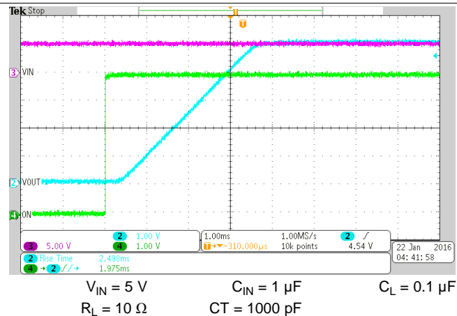
Figure 13. Rise Time ( t_{\text{R}} ) at V_{\text{IN}} = 5 \text{ V}
