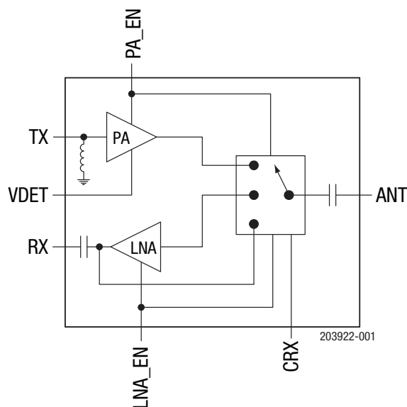
Figure 1. SKY85746-11 Block Diagram
