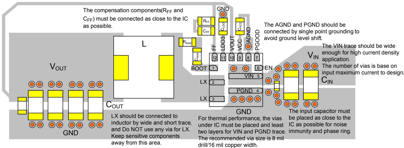
Figure 8. Layout Guide of RT6258B
