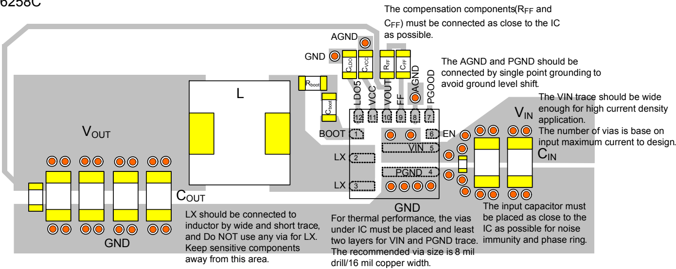
Figure 9. Layout Guide of RT6258C
