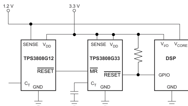
Typical Application
