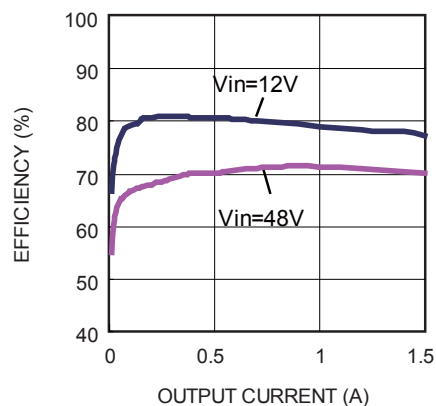
Efficiency @ V_{OUT}=2.5V
