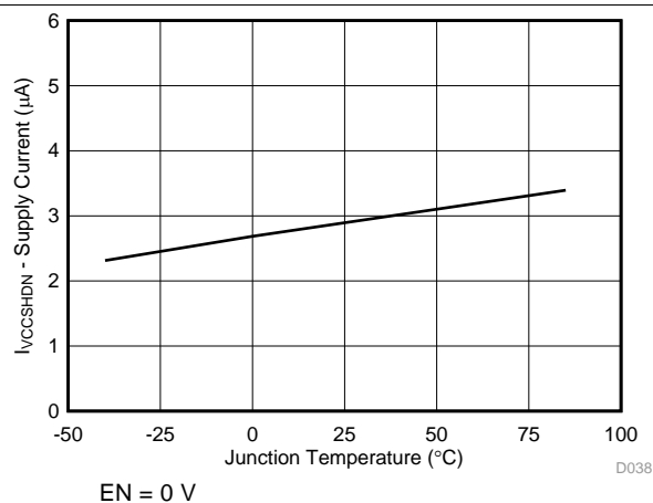
Figure 11. VIN Shutdown Current vs Junction Temperature
